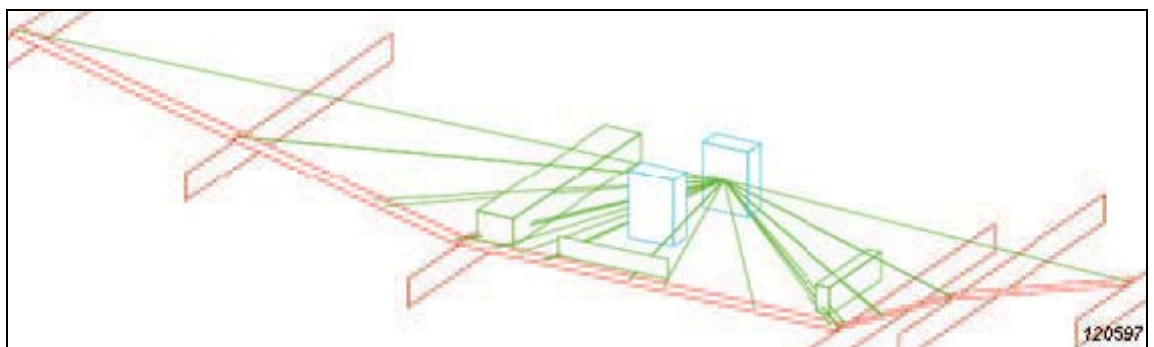
Fig. 1 The method of projection ensures correct segmentation (in 3D) into sections with the same propagation conditions. Results are less sensitive to small changes in receiver point position. These factors lead to more realistic results
